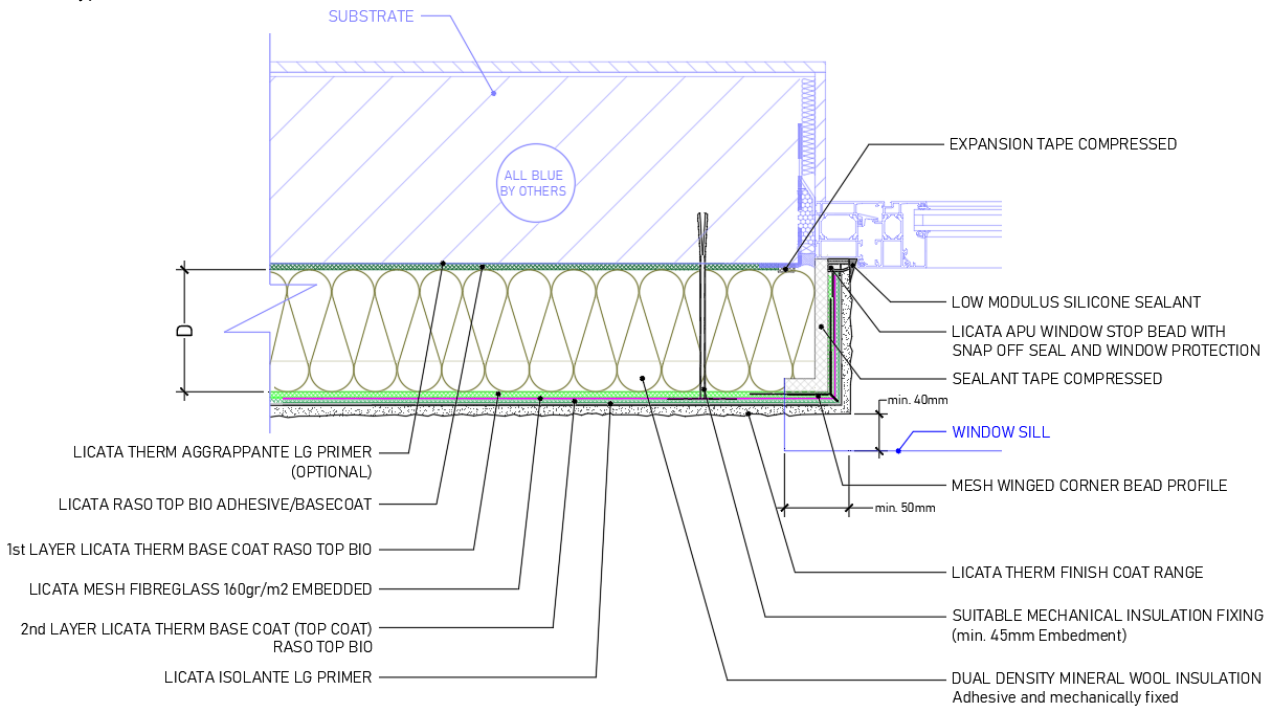
Diagram 5 - Typical window/door reveal detail
