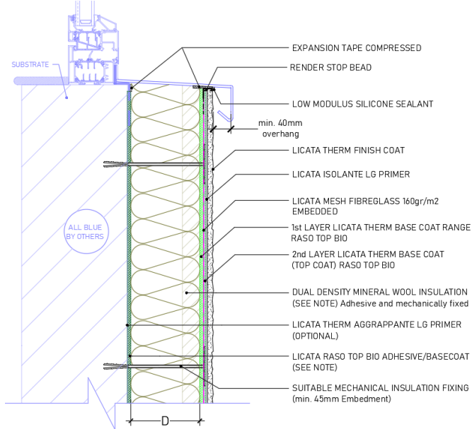
Diagram 6 - Typical window cill detail
