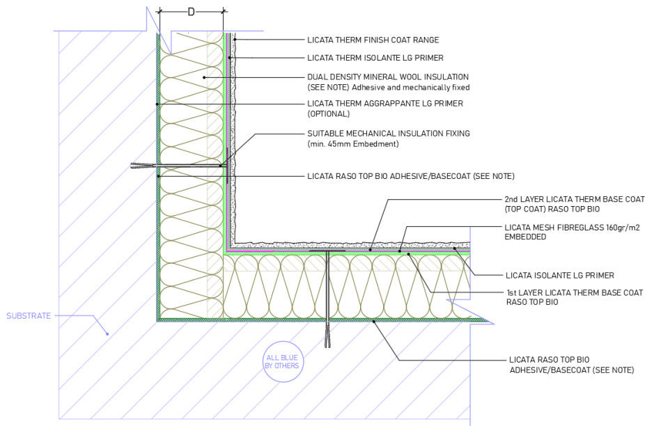
Diagram 3 - Typical internal corner detail
