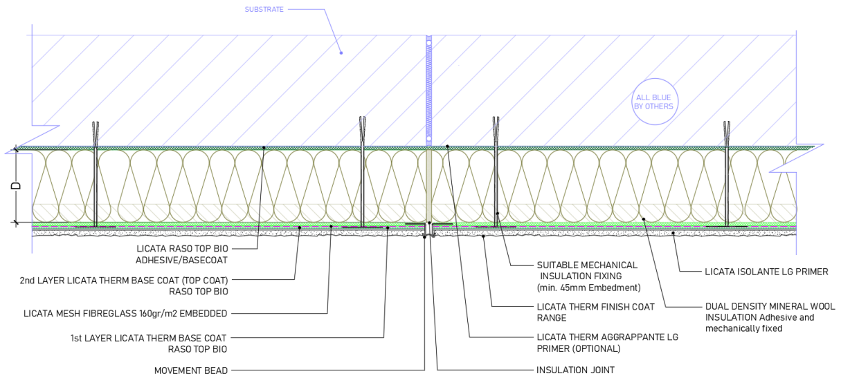
Diagram 2 - Typical vertical movement joint detail
