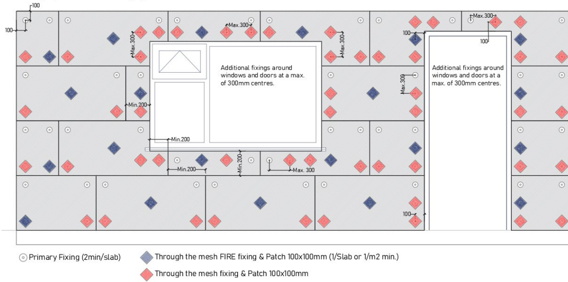
Diagram 1 - Typical fixing pattern
