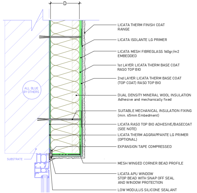
Diagram 7 - Typical window head detail
